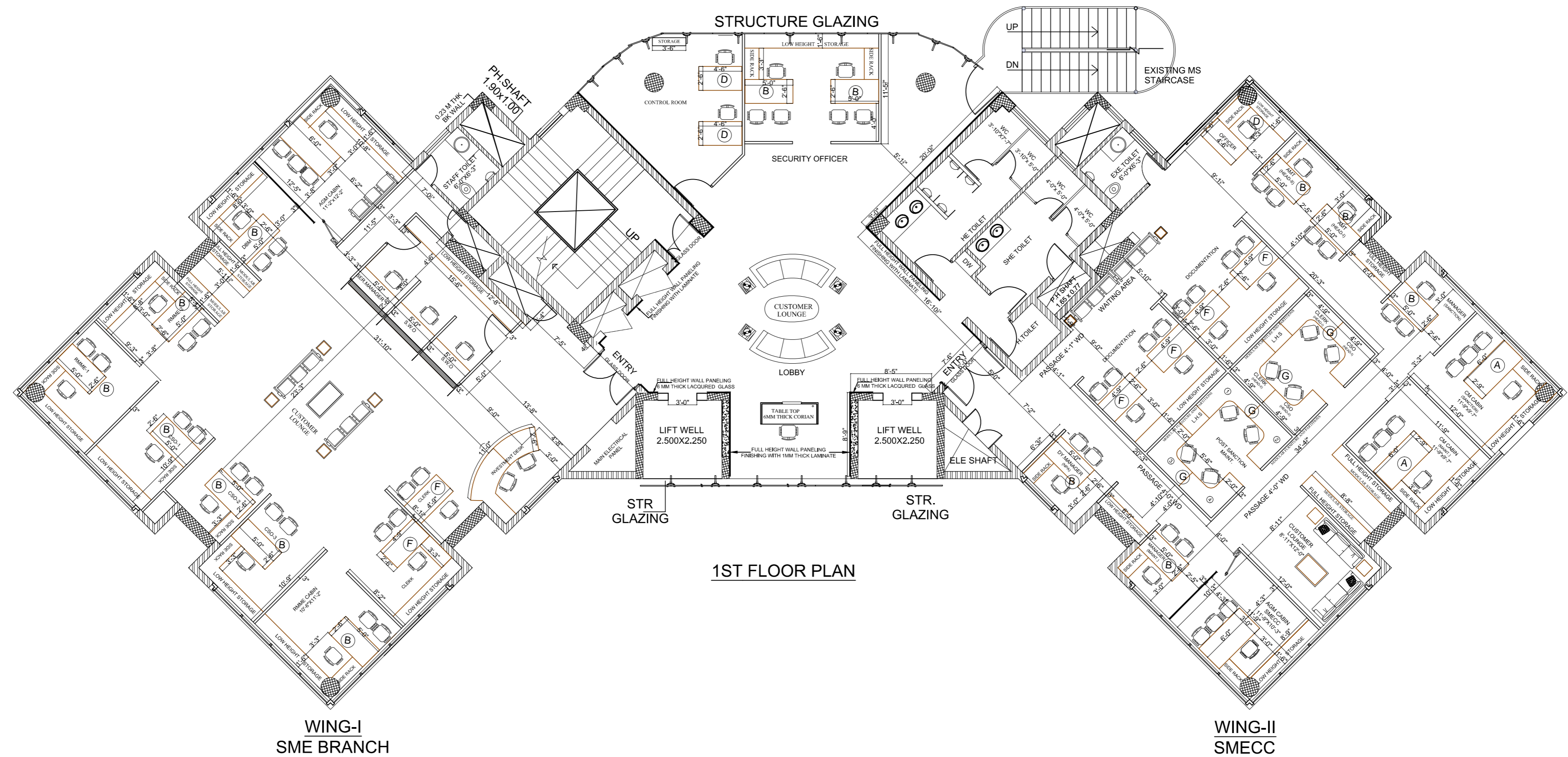
1ST FLOOR PLAN FURNITURE LAYOUT PLAN
